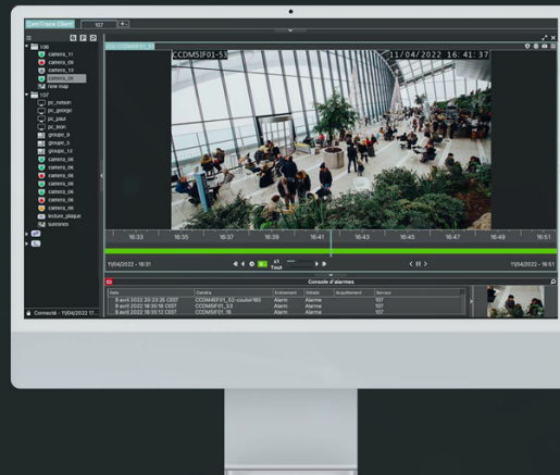
CamTrace Client
