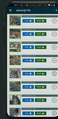
CamTrace Mobile
